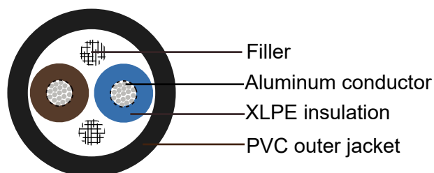
U1000 AR2V
